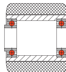
ZZV-ball bearing
