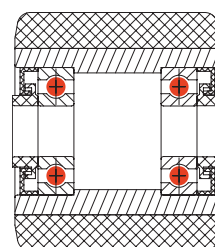
Labyrinth sealing
