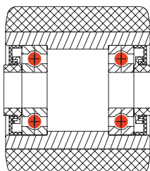
Labyrinth sealing
