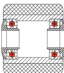
KS-sealing
