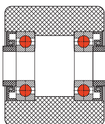
Labyrinth sealing
